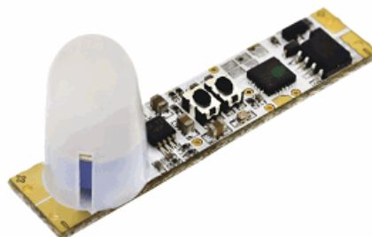
Vypínač do lišt PIR+SOUKRAK LUX 50x10x12/14mm 7,5A 12V DC (90W)
