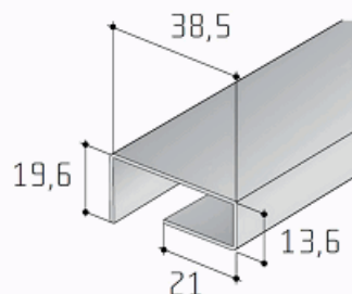
Madlo S41SV01 /S41SV01-J2184/
